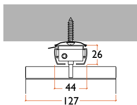
127mm Top Fix
