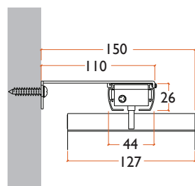
127mm Face Fix
